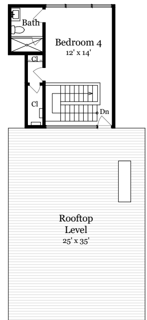
FOURTH FLOOR
